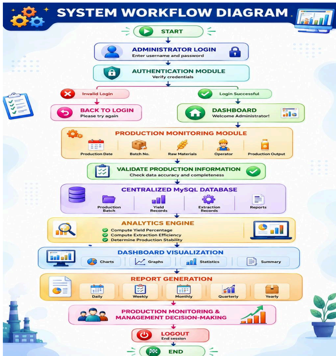
Figure 4.1 illustrates the System Workflow Diagram of the system.
